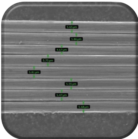
Pyrogasified rCF – SEM image Magnification: 3000×
