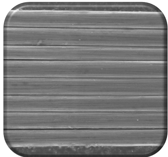
Pyrogasified rCF – SEM image Magnification: 5000×
