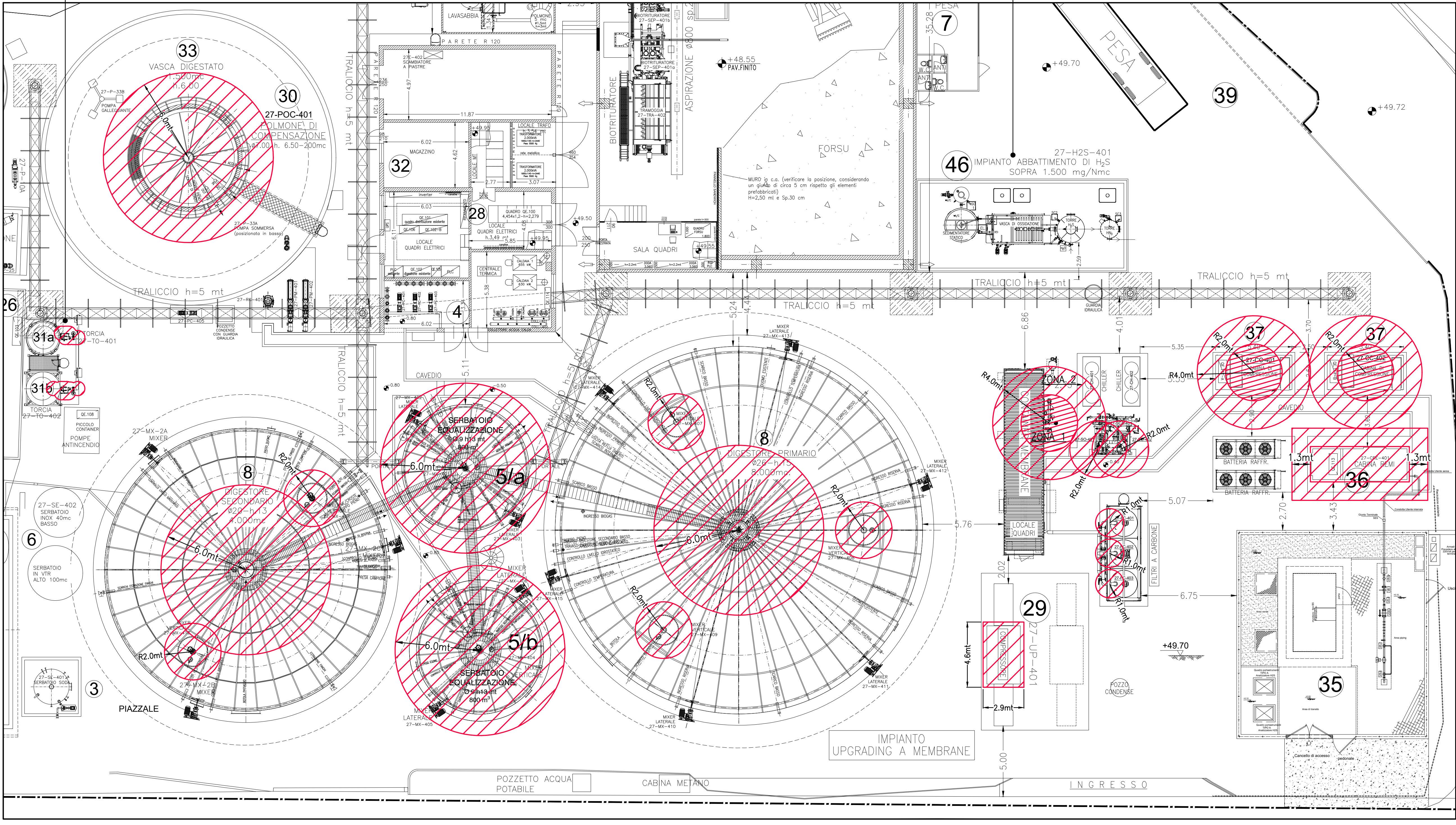
PLANIMETRIA ZONE ATEX Scala 1:150
